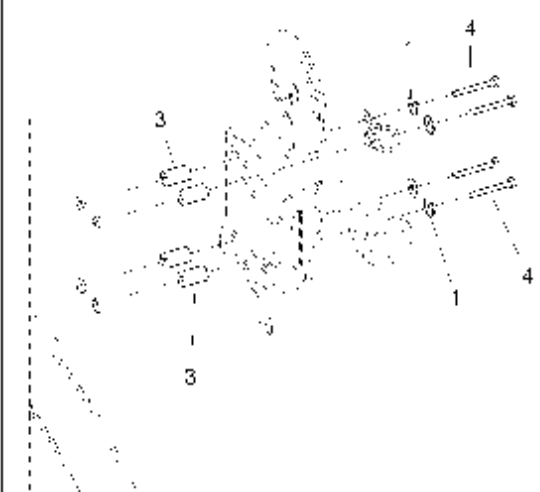
Anbindung an CM 1200 / 1250 / 1600 Connection to CM 1200 / 1250 / 1600
